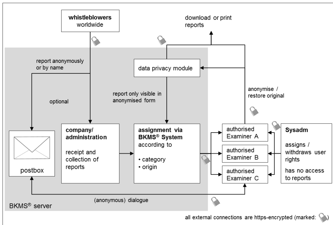
Figure 4: data flow
